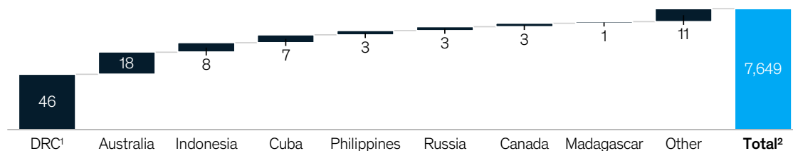
Copper (Cu) reserves, % of Cu contained
