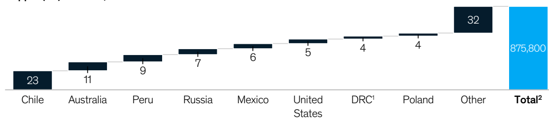
Lithium (Li) reserves, % of Li contained
