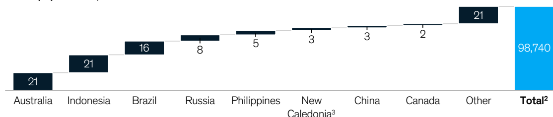
Rare earth elements (REE) reserves, % of REO 4 equivalent
