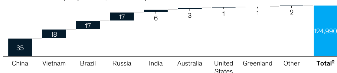
Rare earth elements (REE) reserves, % of REO 4 equivalent
