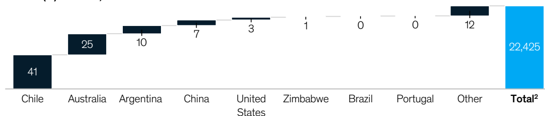
Nickel (Ni) reserves, % of Ni contained
